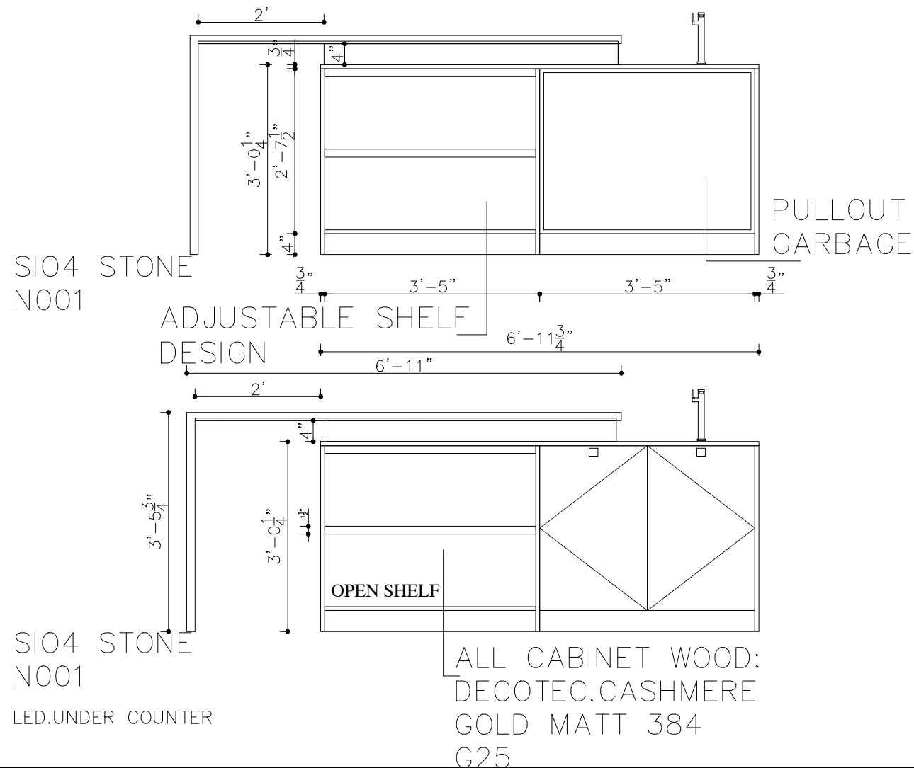
VIEW B
