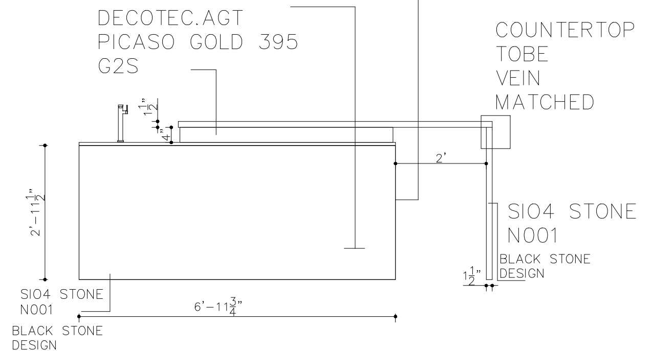
VIEW C
